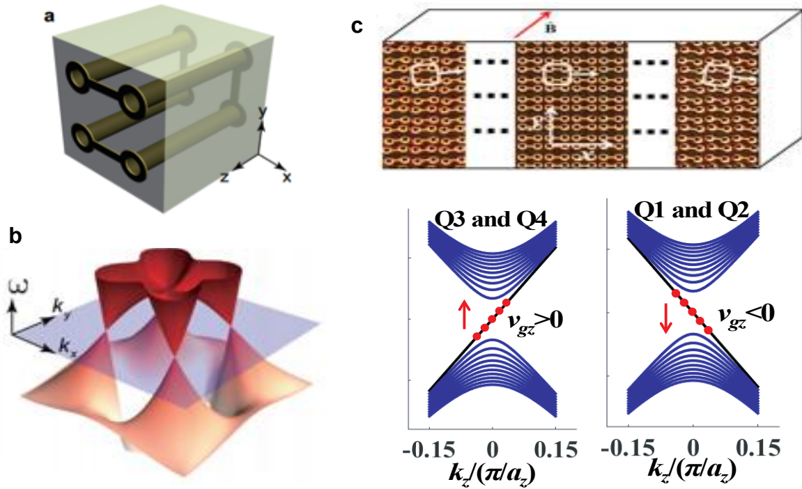
Metamaterials hosting ideal Weyl points in the momentum space. a. the unit cell of the ideal Weyl metamaterial formed by saddle-shaped metallic loop. b. The band structure of metamaterial shows that there are four ideal points located at the same frequency, as protected by the symmetry of the unit cell. c. By introducing inhomogeneity to the ideal Weyl metamaterial, an effective magnetic field can be induced, which leads to formation of chiral zero modes, which are one-way propagating bulk modes.
